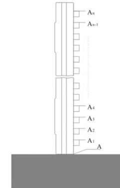
Parallelism II: Parallelism of each working surface and Surface A of inspection surface plate
