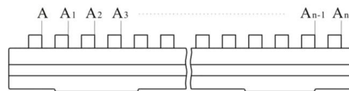
Parallelism I: Parallelism of each working surface and Origin Working Surface A
