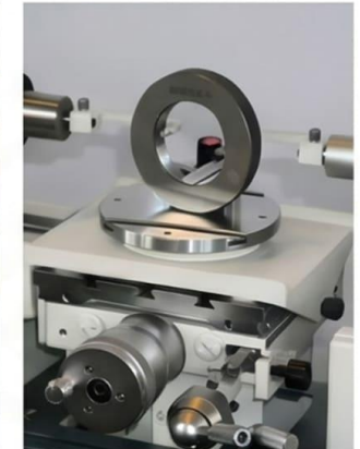
Universal Length Measuring Instrument
